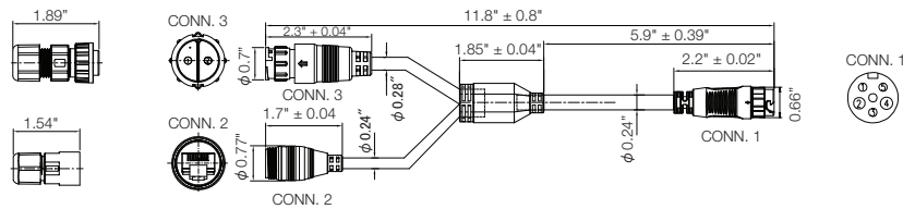
RB RJ45 STARTER Y-CABLE IP67 (AM401000055)
