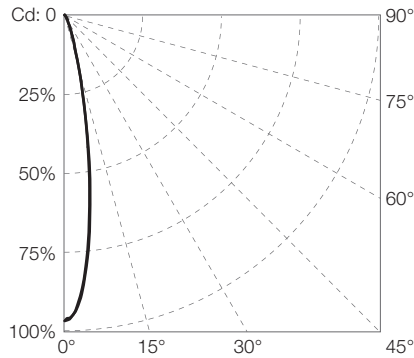
Diagram based on HO 1' RGBW 15°
