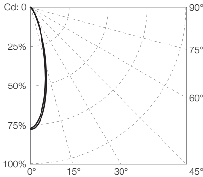
Diagram based on HO 1' RGBW 25°
