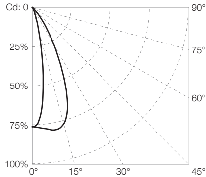
Diagram based on HO 1' RGBW 50° x 30°
