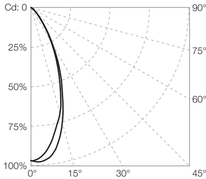
Diagram based on HO 1' RGBW 35°
