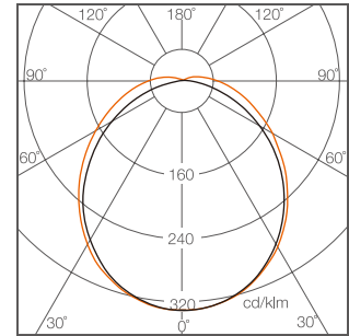
16W, 1200mm
