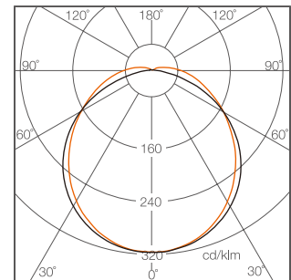
33W, 1200mm
