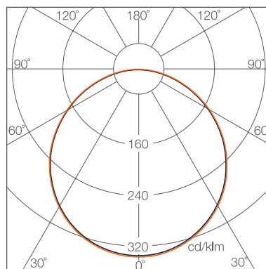
Light Distribution Curve (4000K, 6500K)
